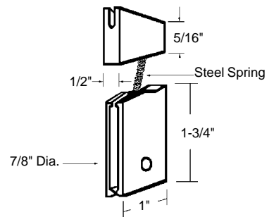
Sliding Screen Door Roller
