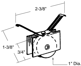
Sliding Screen Door Roller
