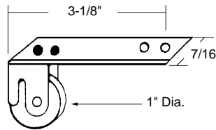
Sliding Screen Door Roller
