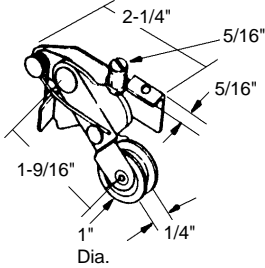
Sliding Screen Door Roller
