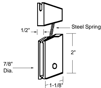
Sliding Screen Door Roller
