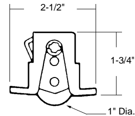
Sliding Screen Door Roller
